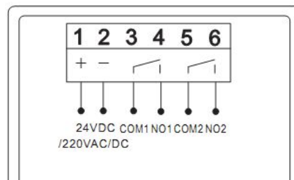
Double Setpoint
